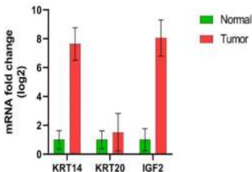
Fig. 1. Fold difference (mean ± SEM) observed with mRNA expression values. Total RNA was isolated from urine cell pellets and cDNAs for IGF2, KRT14, and KRT20 were synthesized. cDNAs were amplified by PCR on a Corbett Rotor-Gene RG-6000 Real-Time PCR Analyzer.
