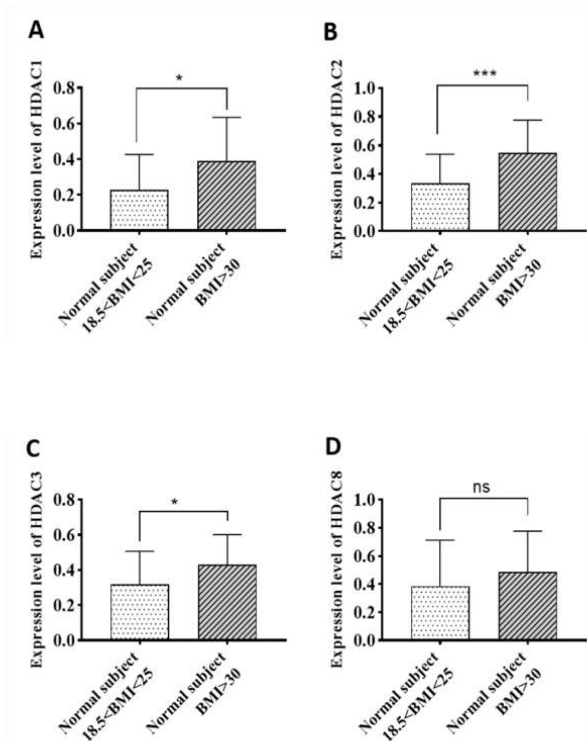
Fig. 2. A. HDAC1 B. HDAC2 C. HDAC3, and D. HDAC8 expressions in normal samples (N) with BMI>30 (obese) compared to normal samples with 18.5<BMI<25 (non-obese). The mean \pm SEM. * P < 0.05; ns: non-significant.
