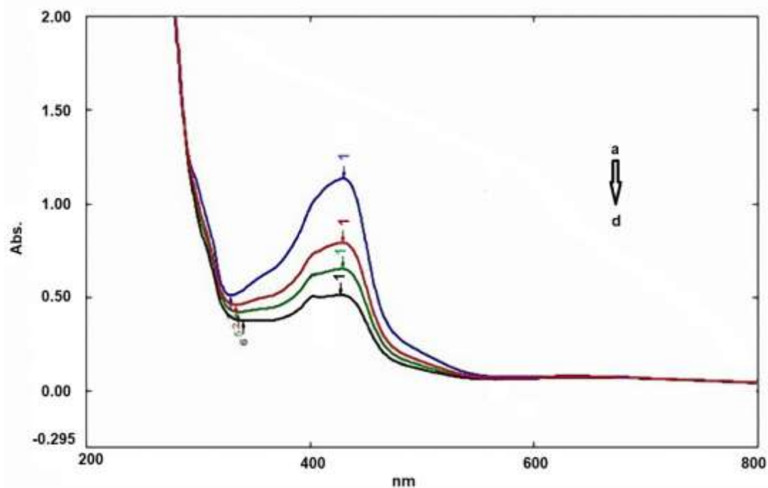
Fig. 2 A spectrophotometric spectrum of the FAS complex. The residual peroxide concentrations were directly proportional to the absorbance of the formed complex: (a) 200 \mu M H_2O_2 ; (b) 125 \mu M H_2O_2 ; (c) 100 \mu M H_2O_2 ; (d) 75 \mu M H_2O_2 .
