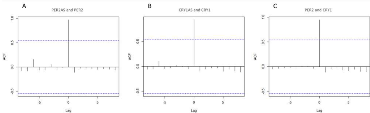
Fig. 2. Cross-correlation analysis between the expression of PER2AS-PER2 , CRY1AS-CRY1 and PER2-CRY1 gene pairs. (A-C) there is the maximum positive correlation for all transcripts at lag= 0. Horizontal dashed line as a threshold line determines the significance level of cross correlation between 2 genes.
