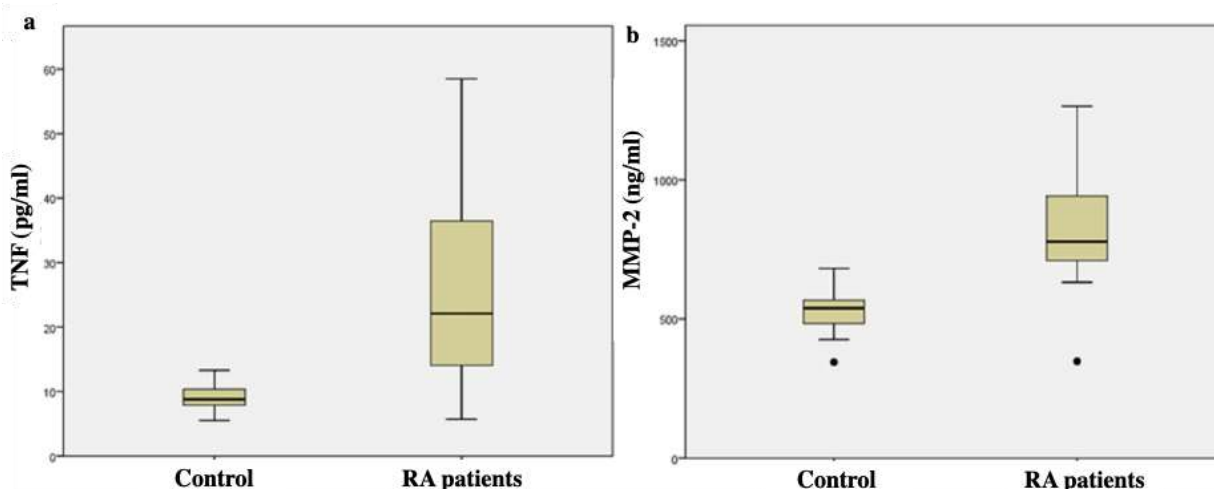
Fig. 1. Relative serum expression of (a) TNF-α (b) and MMP-2 among RA patients and control group.
